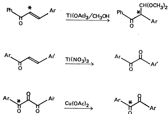
Scheme 1. Ar and Ar' refer to substituted phenyls.
